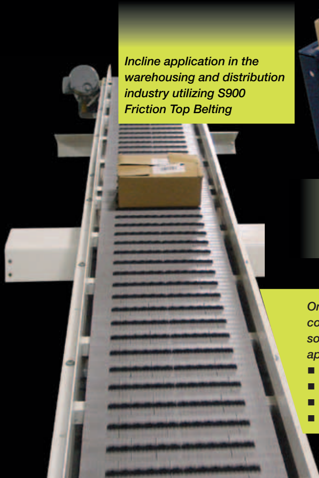
Tight transfer application in material handling industry utilizing S1000 Flat Top Belting with a 1" nosebar
